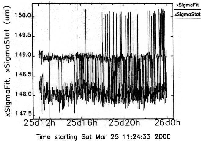
FIGURE 4. A random sample of peak width from the APS data logger over a 12 hour period. Top (xSigmaStat): horizontal beam size derived from the rms calculations. Bottom (xSigmaFit): the horizontal beam size derived from the Gaussian fit.
