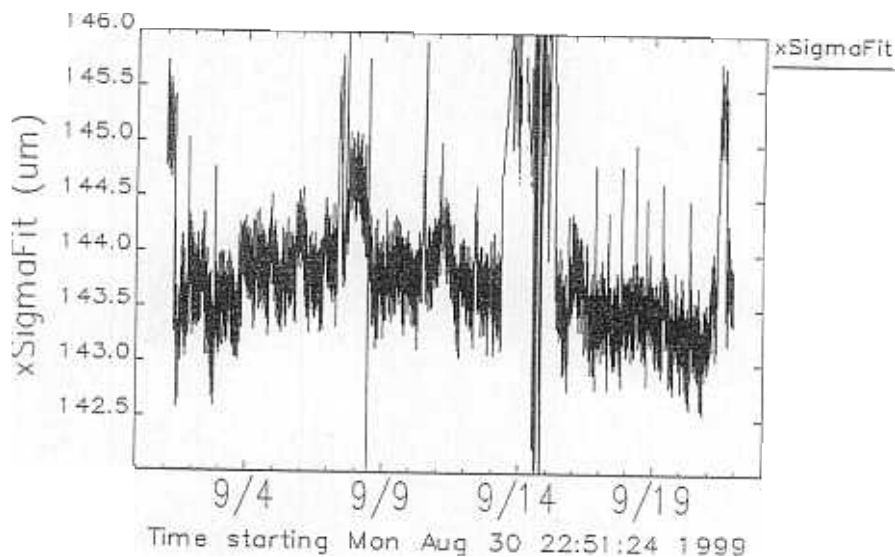
FIGURE 6. The rms horizontal beam size (measured at 1 Hz bandwidth, recorded at 1 minute interval) during September 1999 recorded by the APS data logger. Significant variations can be seen during machine studies on September 1, 7, 14-15, and 21.
