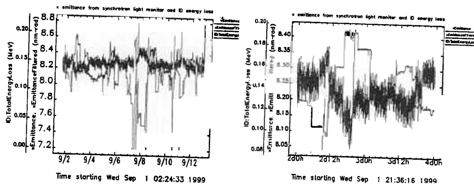
FIGURE 7. The horizontal beam emittance in the first two weeks (A) and first two days (B) during September 1999 recorded by the APS data logger. The total energy loss in the APS insertion devices is also plotted (thin lines).
