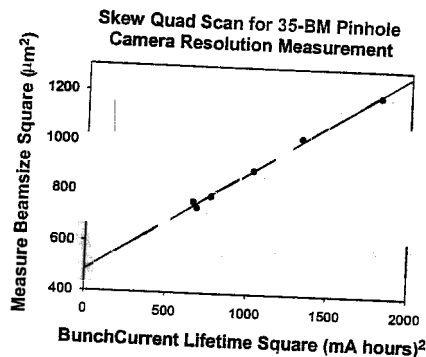
FIGURE 5. Resolution characterization with lifetime measurement vs. vertical beam size. Extrapolation to the zero lifetime, with known lifetime-beam size dependence, gives the total camera resolution of 22 \mu\text{m} .
