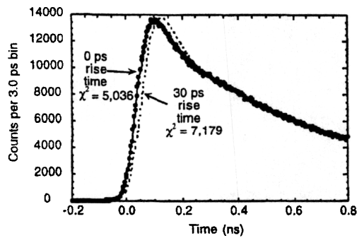
Figure 5. Data and best fit curves for a BaF 2 2 x 10 x 10 mm crystal painted black on 5 sides. See text for details.
