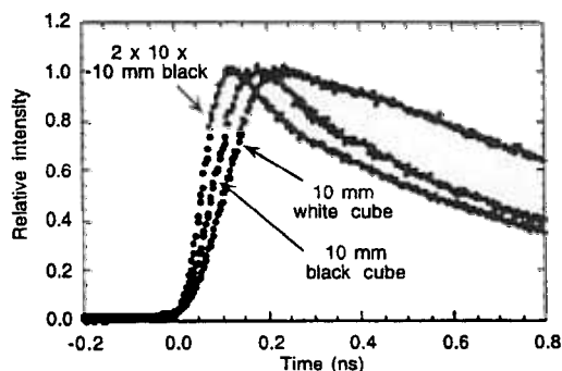
Figure 2. Normalized fluorescence time spectra from three \text{BaF}_2 crystals of different sizes and surface reflectors.
