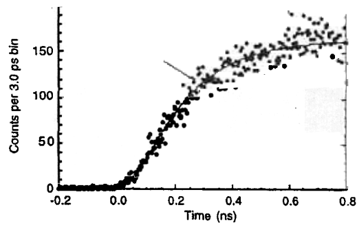
Figure 6. YAlO 3 :Ce 10-mm cube painted black on five sides. Best fit rise time is 240 ps.
