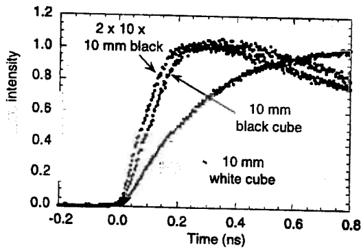
Figure 3. Normalized fluorescence time spectra from three \text{PbWO}_4 crystals of different sizes and surface reflectors.
