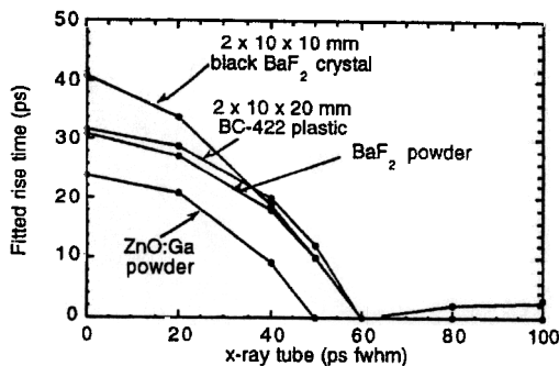
Figure 4. Fitted rise time vs. fwhm of Gaussian used to simulate the time response of the x-ray tube.
