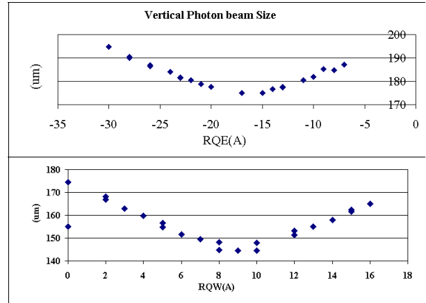
Figure 5: rms of gaussian fits after deconvolution by diffraction function, while scanning the two families of skew quadrupoles
