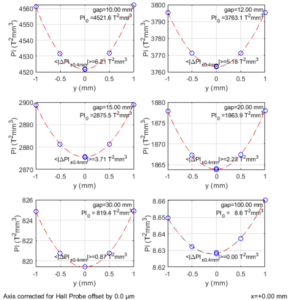
SXPS_16346_DATASET0002_Final_Results_Z_Scans
