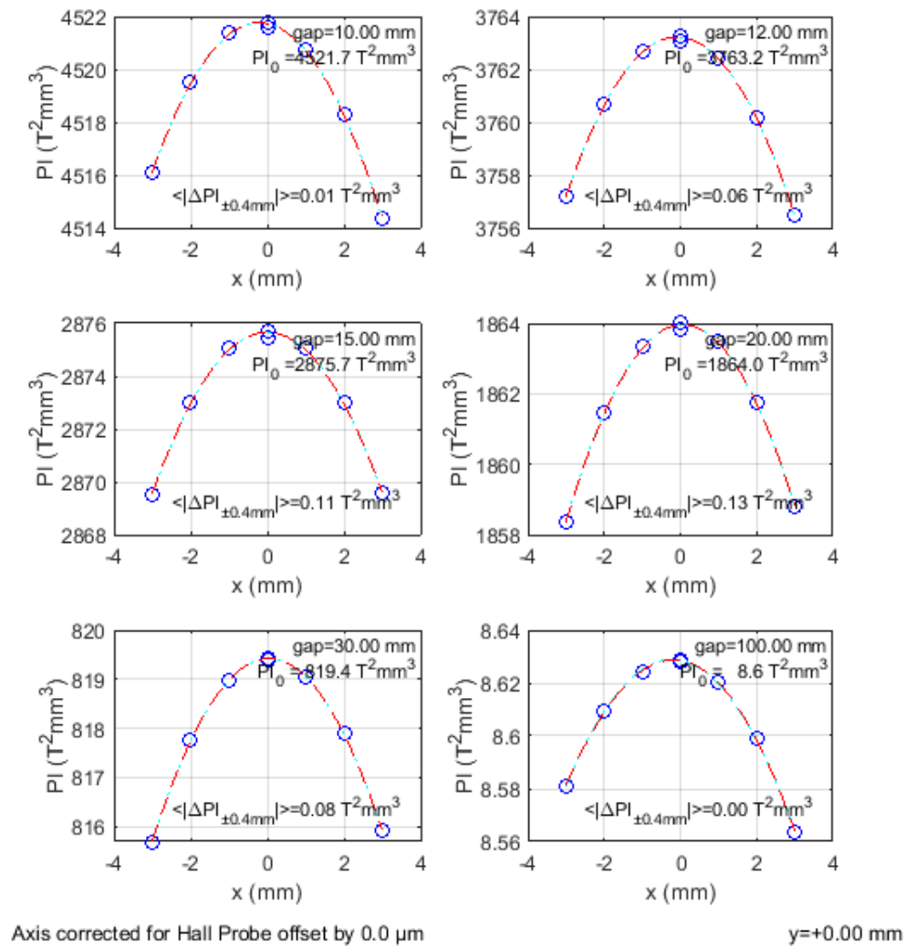
SXPS_16346_DATASET0002_Final_Results_Z_Scans
