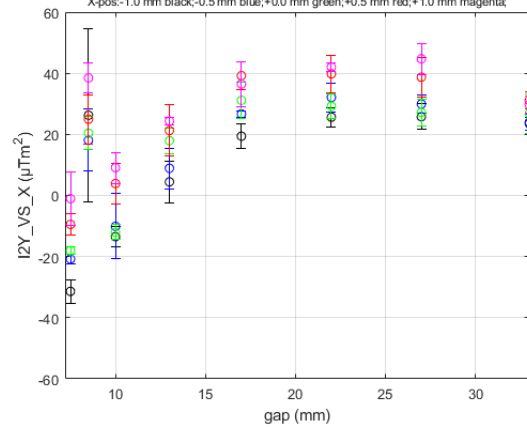
I2Y_VS_X for HE_SXU-022 at Long Coil/GoodFieldRegion DATASET0001
