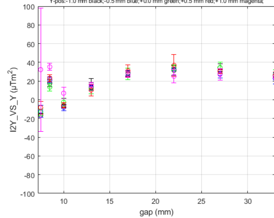
I2Y_VS_Y for HE_SXU-022 at Long Coil/GoodFieldRegion DATASET0001
