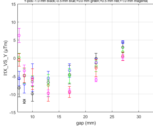
I1X_VS_Y for HE_SXU-022 at Long Coil/GoodFieldRegion DATASET0001
