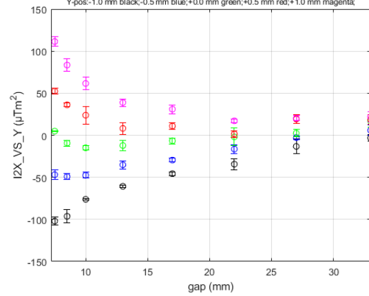
I2X_VS_Y for HE_SXU-022 at Long Coil/GoodFieldRegion DATASET0001
