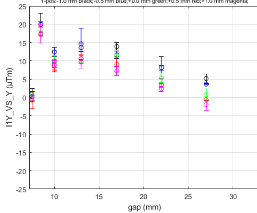
I1Y_VS_Y for HE_SXU-022 at Long Coil/GoodFieldRegion DATASET0001
