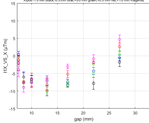
I1X_VS_X for HE_SXU-022 at Long Coil/GoodFieldRegion DATASET0001
