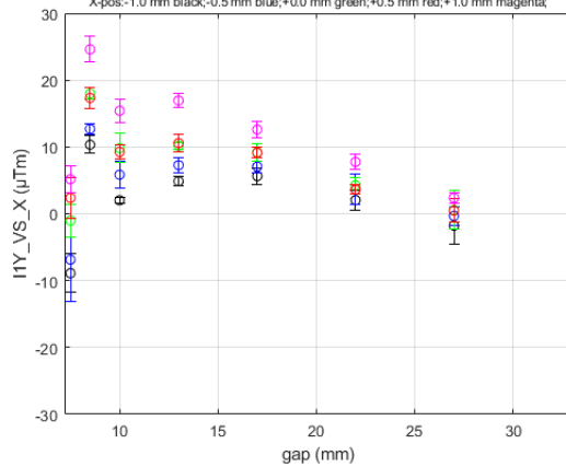
I1Y_VS_X for HE_SXU-022 at Long Coil/GoodFieldRegion DATASET0001
