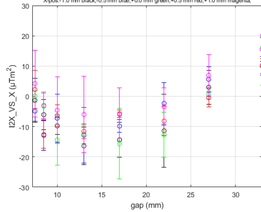
I2X_VS_X for HE_SXU-022 at Long Coil/GoodFieldRegion DATASET0001
