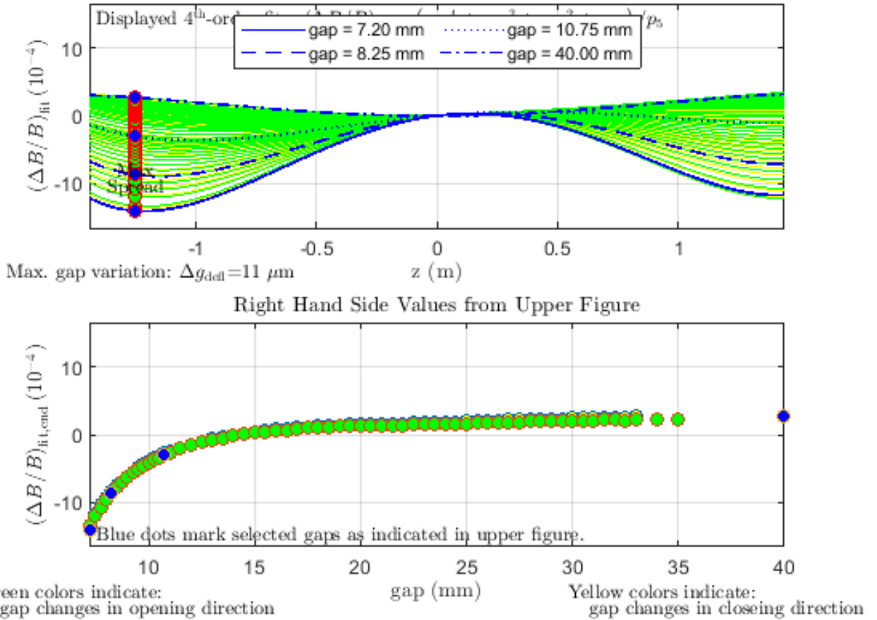
HE_SXU.009_DATASET0001_Final_Results_Z_Scans_ZeroTaper Fitted Undulator Field Peaks for Various Undulator Gaps
