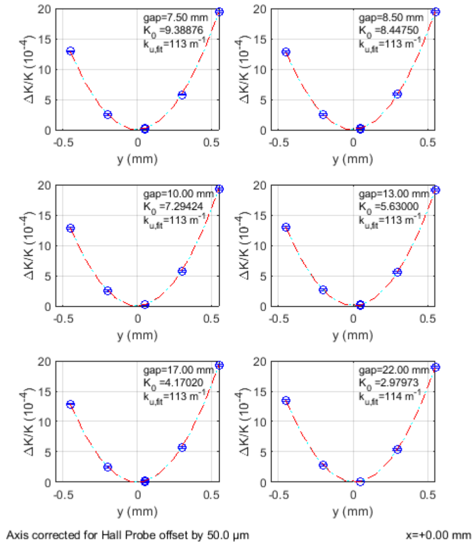
HE_SXU_001_DATASET0001_Final_Results_Z_Scans
