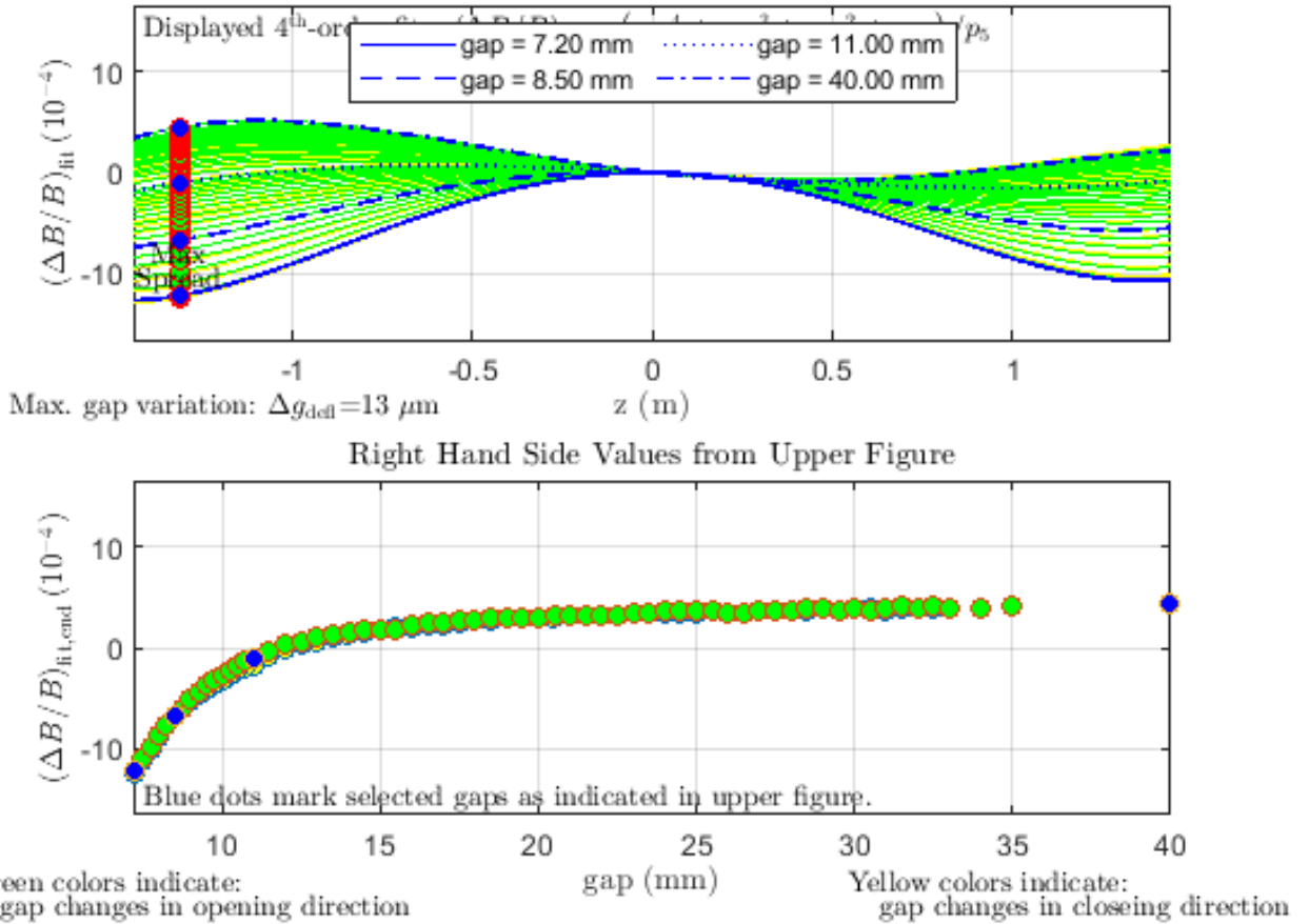
HE_SXU.001_DATASET0001_Final_Results_Z_Scans_ZeroTaper Fitted Undulator Field Peaks for Various Undulator Gaps
