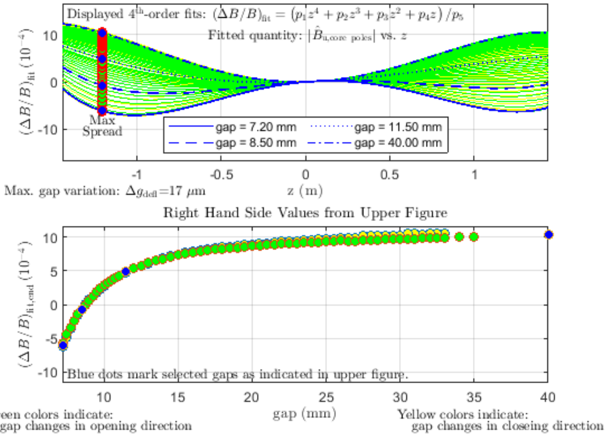
HE_SXU_030_DATASET0001_Final_Results_Z_Scans_ZeroTaper Fitted Undulator Field Peaks for Various Undulator Gaps
