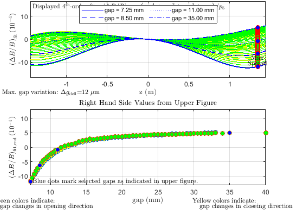
HE_SXU.012_DATASET0001_Final_Results_Z_Scans_ZeroTaper Fitted Undulator Field Peaks for Various Undulator Gaps
