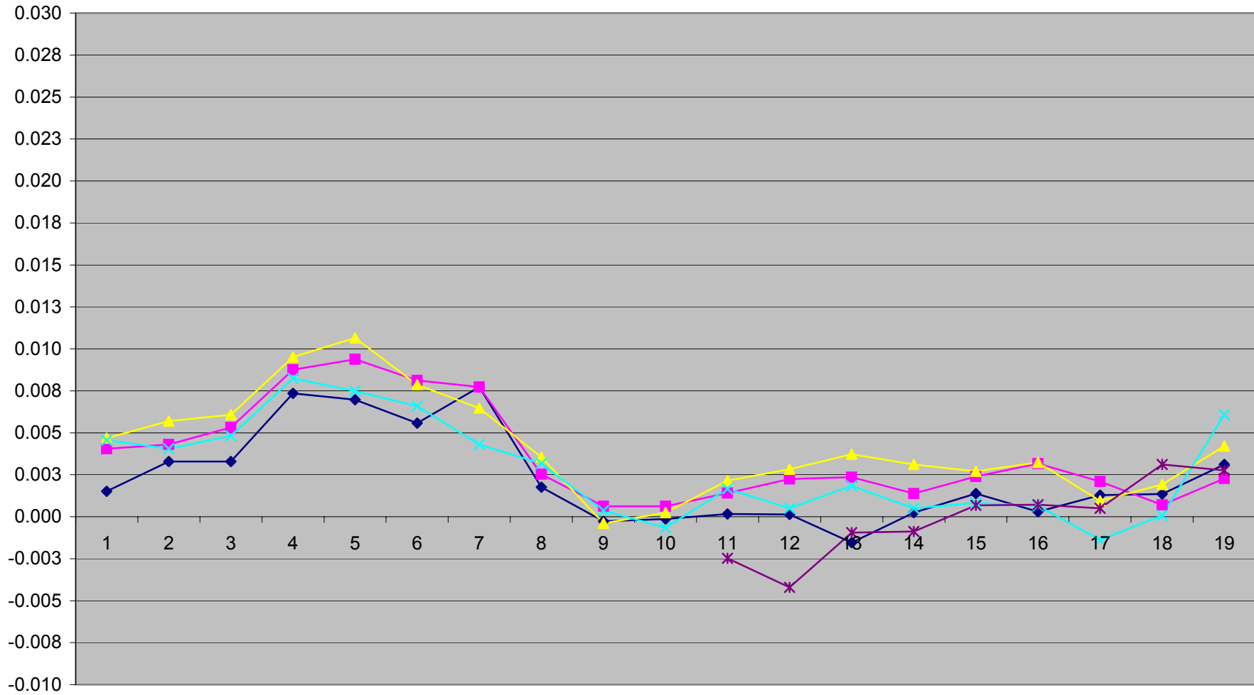
Quadrant 1 Floor Elevation in Meters from Ideal - 06/18/03 Check on Previous Survey - 2 Ft Intervals
