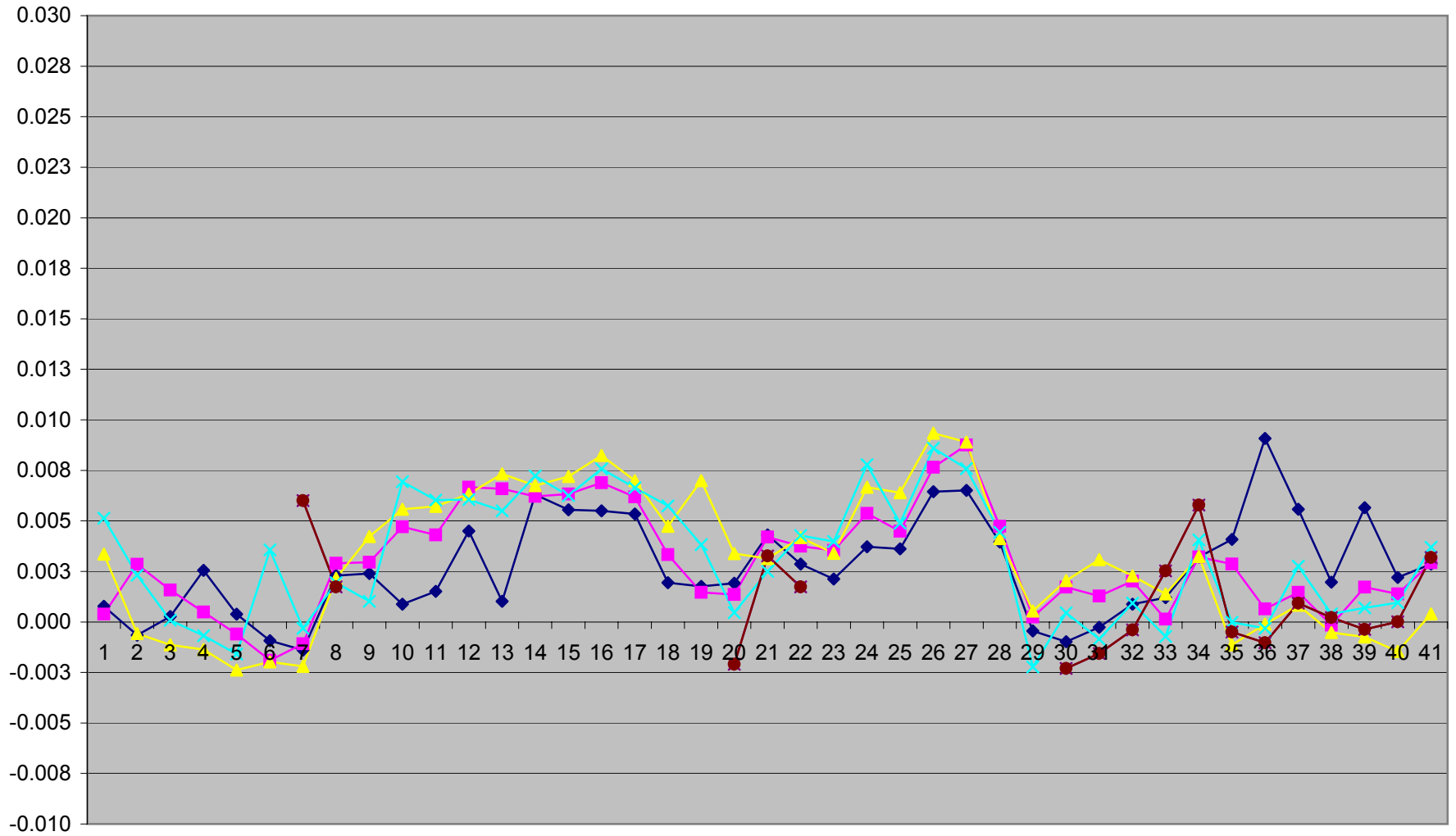
Quadrant 1 Floor Elevation in Meters from Ideal - 06/17/03,06/18/03
