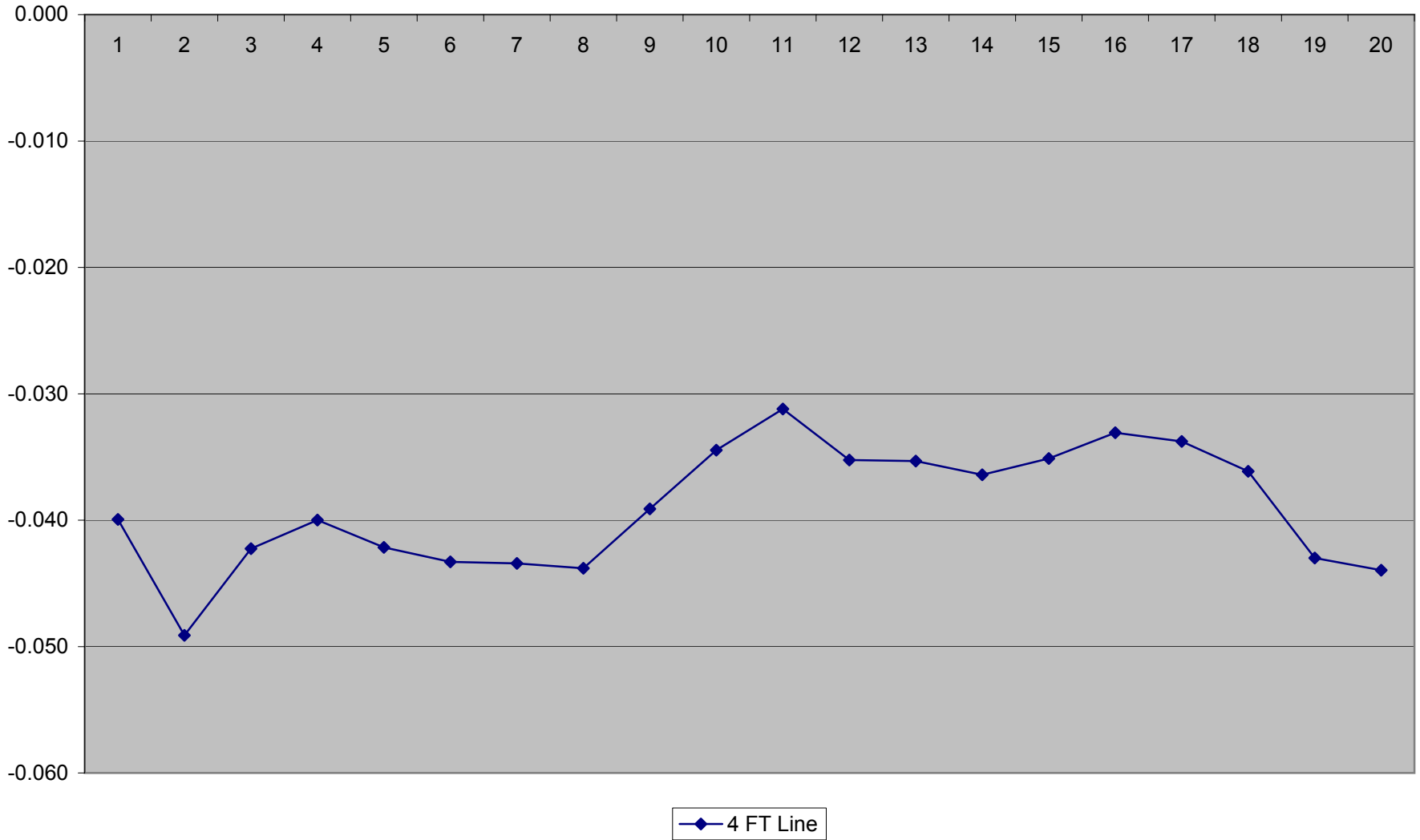
West Pit Floor Elevation in meters from Ideal - 06/18/03 4 FT Line from Outside Wall, 2 Ft Intervals
