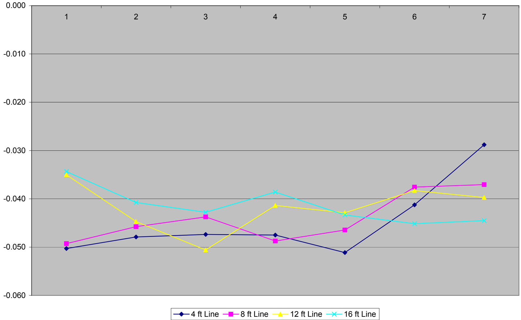
East Pit Floor Elevation in meters from Ideal 6/5/03
