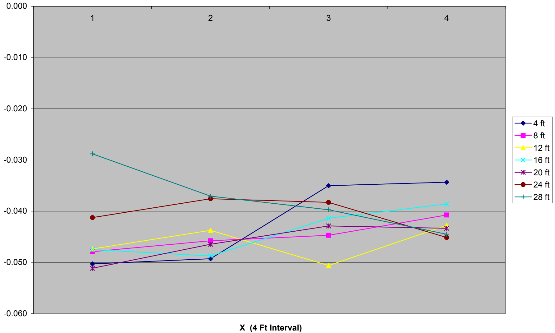
East Pit Cross Section Floor Elevation in meters from Ideal 6/4/03
