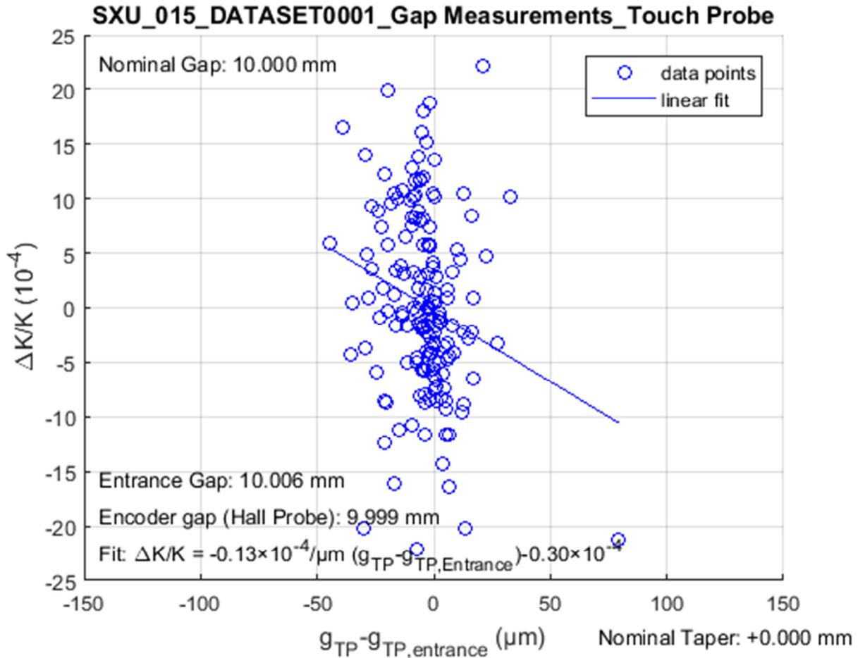
The figure shows the correlation between the \Delta K_u/K_u for each pole from Hall probe measurements for the tuning gap and the deviation of the pole gap measured by the touch probe relative to its average (for the 164 core poles). The average gap measured with the touch probe and the one measured with the gap encoder are shown in the lower left corner of the figure. Also shown is the fit function.
