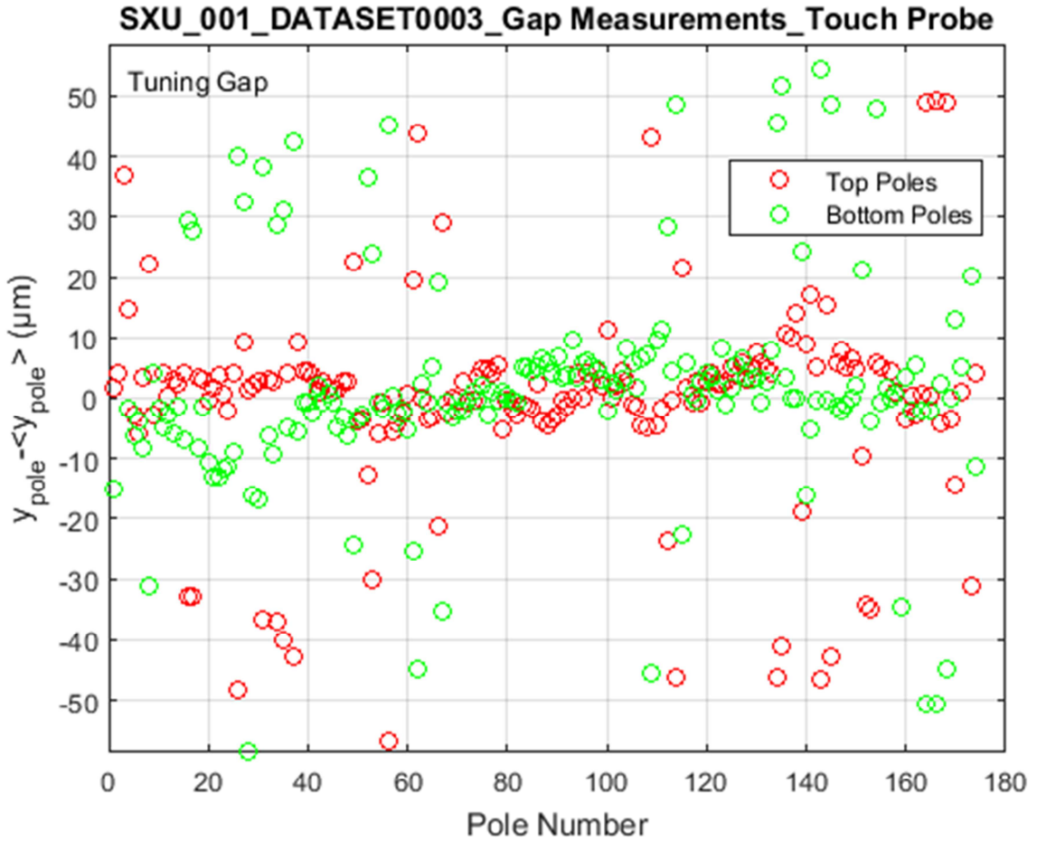
The figure shows the relative vertical positions of the center of each pole (top red, bottom green) relative to the horizontal plane defined by the Kugler bench at the Tuning Gap for all 174 poles, measured by the touch probe. Note: The right most upper magnet module appears to be mounted too high by almost 10 μm relative to the others.
