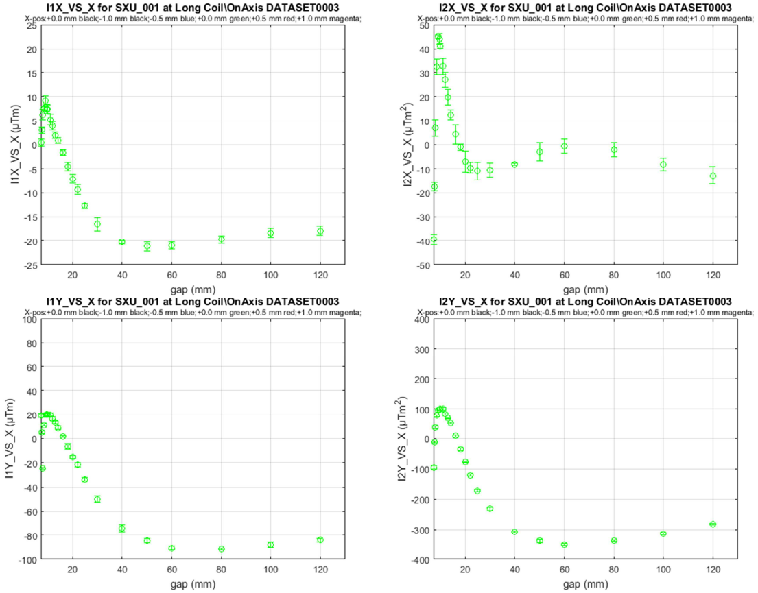
The figure shows the field integrals obtained from long coil measurements on-axis. The vertical axes extend over the tolerance range. All integrals are in tolerance.
