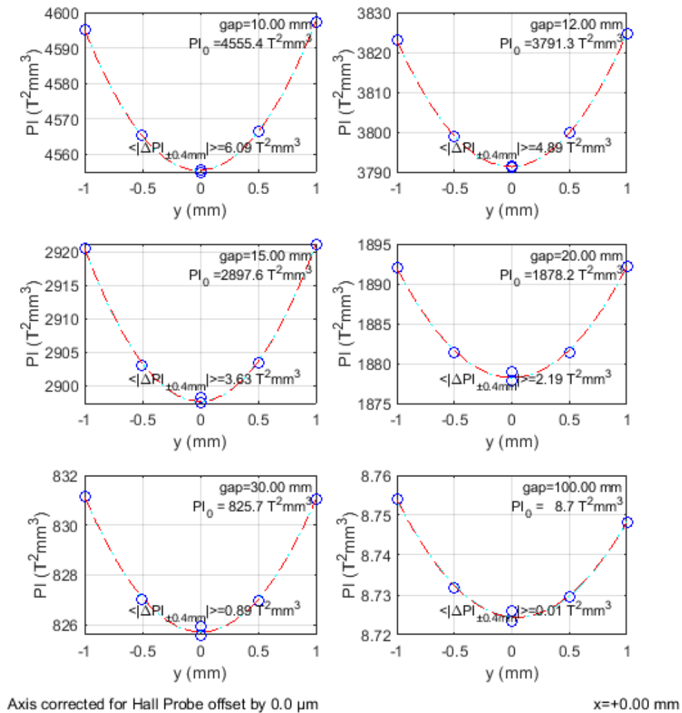
SXPS_16336_DATASET0003_Final_Results_Z_Scans
