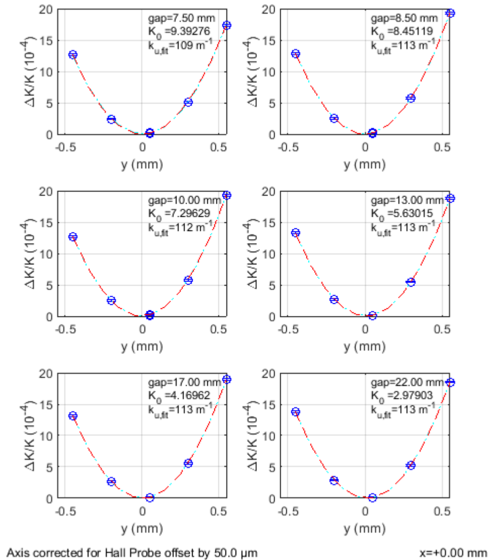
HE_SXU_027_DATASET0001_Final_Results_Z_Scans
