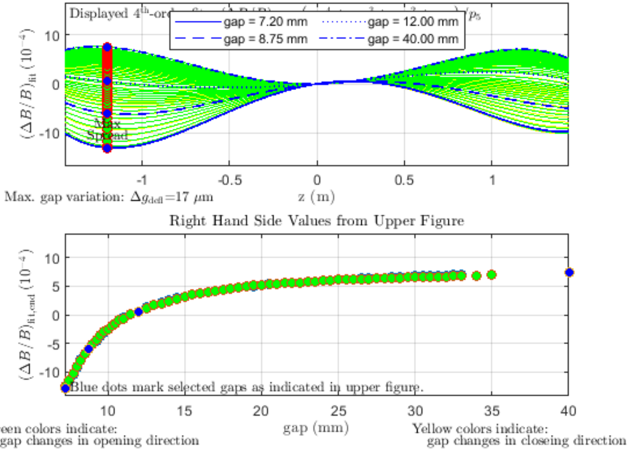
HE_SXU.027_DATASET0001_Final_Results_Z_Scans_ZeroTaper Fitted Undulator Field Peaks for Various Undulator Gaps
