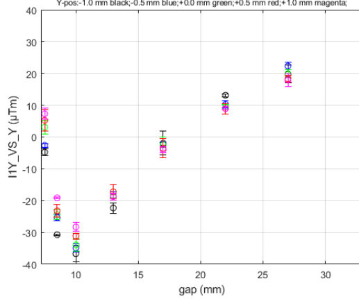
11Y_VS_Y for HE_SXU-020 at Long Coil GoodFieldRegion DATASET0001
