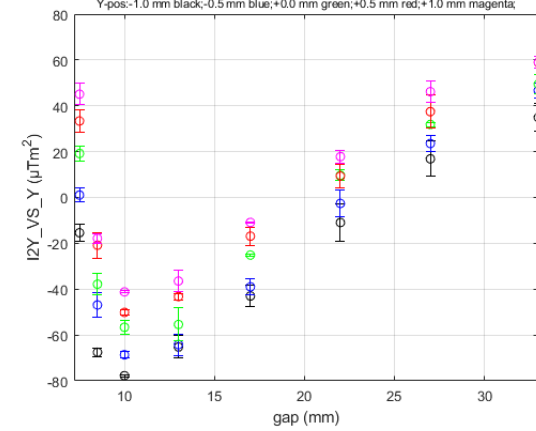
12Y_VS_Y for HE_SXU-020 at Long Coil GoodFieldRegion DATASET0001
