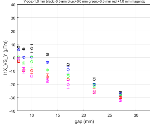
11X_VS_Y for HE_SXU-020 at Long Coil GoodFieldRegion DATASET0001
