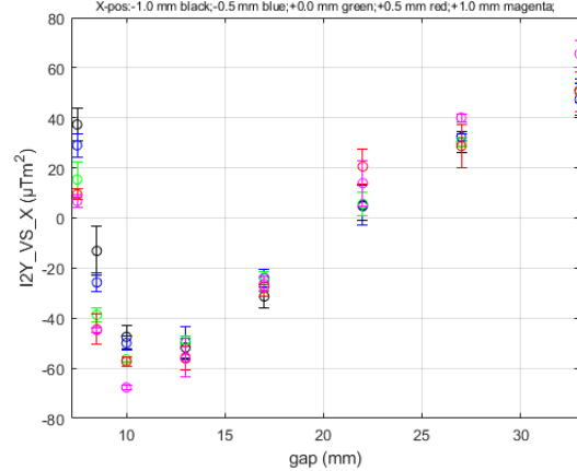
I2Y_VS_X for HE_SXU-020 at Long Coil/GoodFieldRegion DATASET0001
