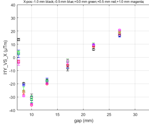
I1Y_VS_X for HE_SXU-020 at Long Coil/GoodFieldRegion DATASET0001
