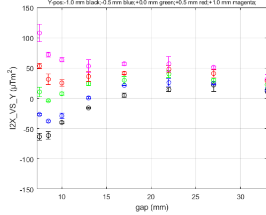
12X_VS_Y for HE_SXU-020 at Long Coil GoodFieldRegion DATASET0001
