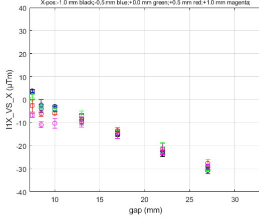
I1X_VS_X for HE_SXU-020 at Long Coil/GoodFieldRegion DATASET0001
