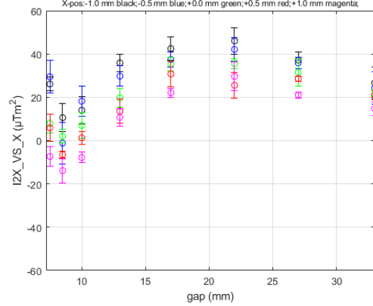
I2X_VS_X for HE_SXU-020 at Long Coil/GoodFieldRegion DATASET0001
