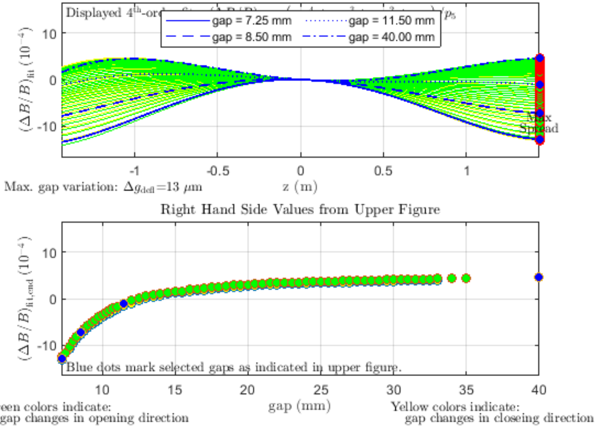
HE_SXU.010_DATASET0001_Final_Results_Z_Scans_ZeroTaper Fitted Undulator Field Peaks for Various Undulator Gaps
