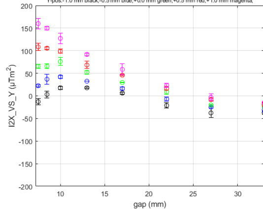
I2X_VS_Y for HE_SXU-006 at Long Coil/GoodFieldRegion DATASET0001
