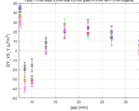
I2Y_VS_Y for HE_SXU-006 at Long Coil/GoodFieldRegion DATASET0001
