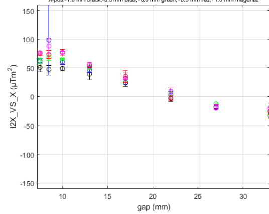
I2X_VS_X for HE_SXU-006 at Long Coil/GoodFieldRegion DATASET0001
