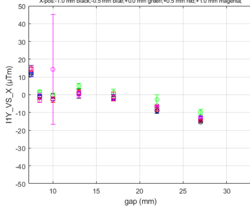
I1Y_VS_X for HE_SXU-006 at Long Coil/GoodFieldRegion DATASET0001
