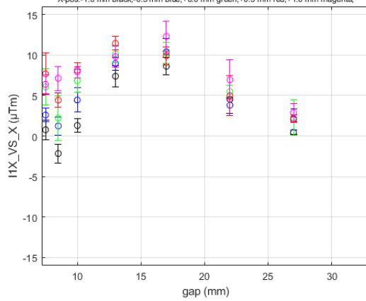
I1X_VS_X for HE_SXU-006 at Long Coil/GoodFieldRegion DATASET0001
