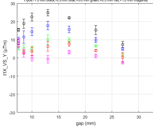
I1X_VS_Y for HE_SXU-006 at Long Coil/GoodFieldRegion DATASET0001
