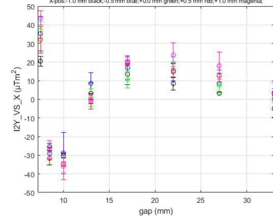
I2Y_VS_X for HE_SXU-006 at Long Coil/GoodFieldRegion DATASET0001
