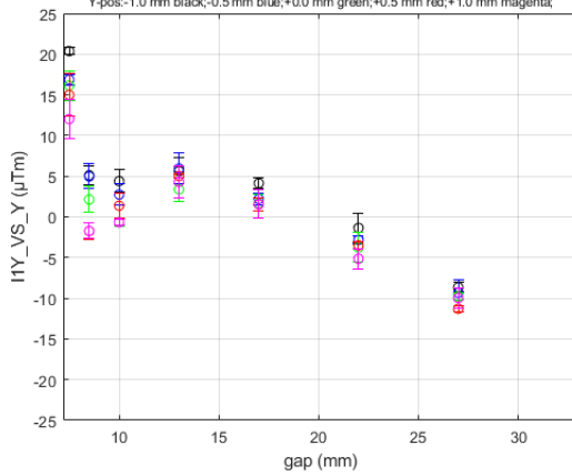
I1Y_VS_Y for HE_SXU-006 at Long Coil/GoodFieldRegion DATASET0001
