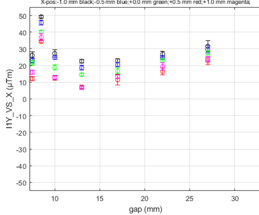
I1Y_VS_X for HE_SXU-002 at Long Coil/GoodFieldRegion DATASET0001
