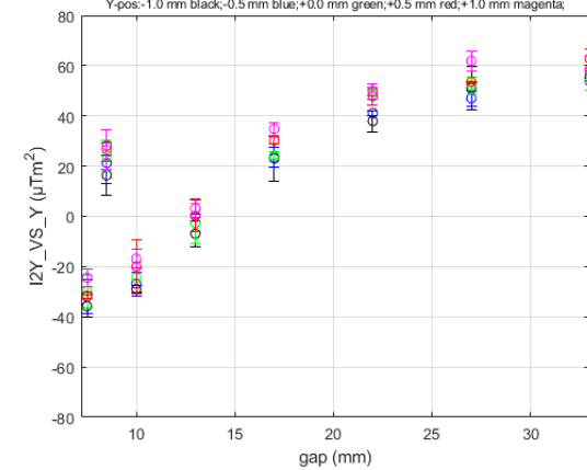
I2Y_VS_Y for HE_SXU-002 at Long Coil/GoodFieldRegion DATASET0001
