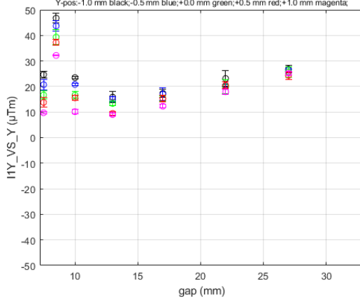
I1Y_VS_Y for HE_SXU-002 at Long Coil/GoodFieldRegion DATASET0001
