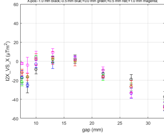
I2X_VS_X for HE_SXU-002 at Long Coil/GoodFieldRegion DATASET0001
