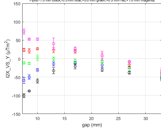
I2X_VS_Y for HE_SXU-002 at Long Coil/GoodFieldRegion DATASET0001
