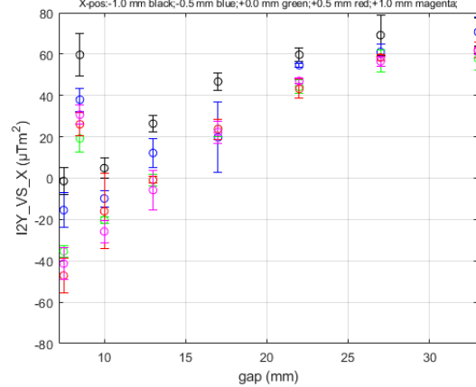
I2Y_VS_X for HE_SXU-002 at Long Coil/GoodFieldRegion DATASET0001
