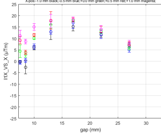
I1X_VS_X for HE_SXU-002 at Long Coil/GoodFieldRegion DATASET0001
