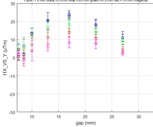
I1X_VS_Y for HE_SXU-002 at Long Coil/GoodFieldRegion DATASET0001
