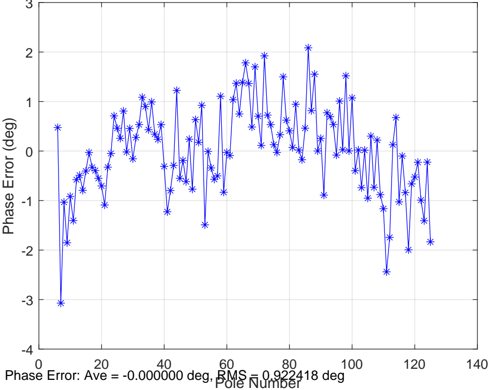
Phase Error At Field Peaks vs Pole Number, No Ends
