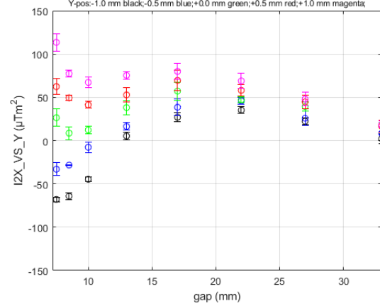
I2X_VS_Y for HE_SXU-019 at Long Coil/GoodFieldRegion DATASET0001
