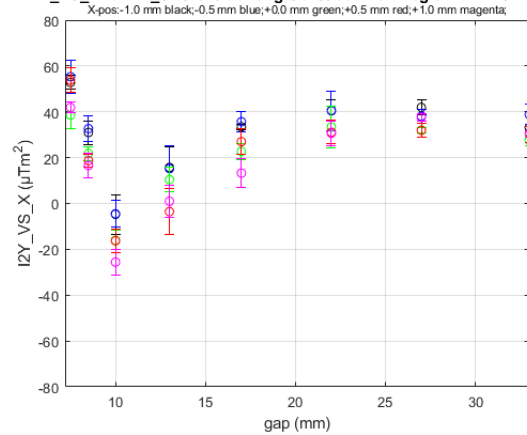
I2Y_VS_X for HE_SXU-019 at Long Coil/GoodFieldRegion DATASET0001
