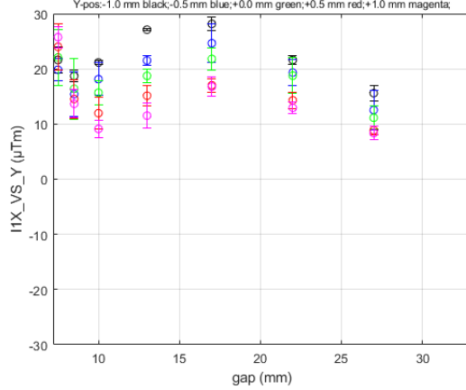
I1X_VS_Y for HE_SXU-019 at Long Coil/GoodFieldRegion DATASET0001
