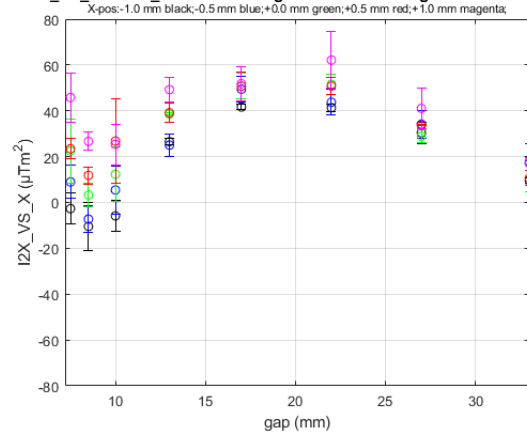
I2X_VS_X for HE_SXU-019 at Long Coil/GoodFieldRegion DATASET0001
