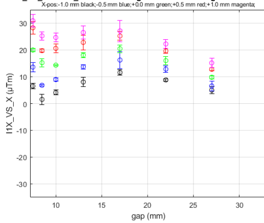
I1X_VS_X for HE_SXU-019 at Long Coil/GoodFieldRegion DATASET0001
