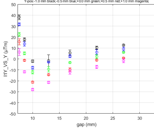
I1Y_VS_Y for HE_SXU-019 at Long Coil/GoodFieldRegion DATASET0001
