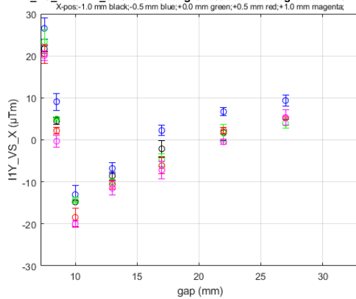
I1Y_VS_X for HE_SXU-019 at Long Coil/GoodFieldRegion DATASET0001
