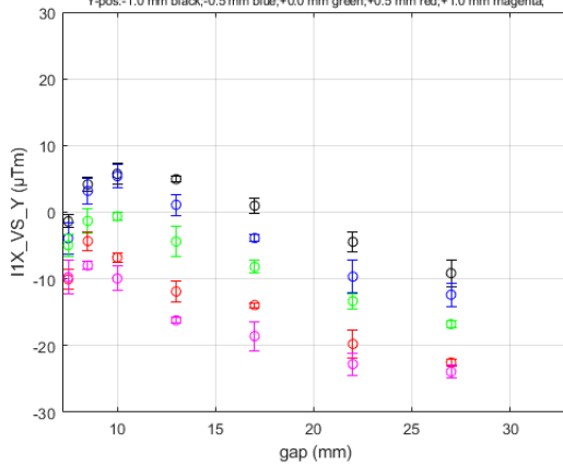
I1X_VS_Y for HE_SXU-011 at Long Coil GoodFieldRegion DATASET0001
