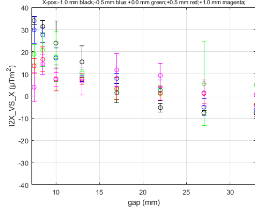
I2X_VS_X for HE_SXU-011 at Long Coil/GoodFieldRegion DATASET0001
