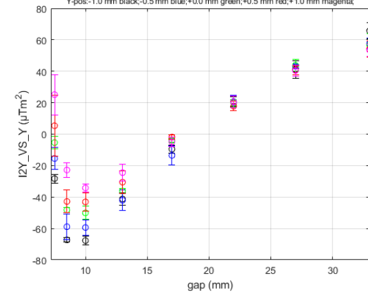
I2Y_VS_Y for HE_SXU-011 at Long Coil GoodFieldRegion DATASET0001
