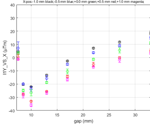
I1Y_VS_X for HE_SXU-011 at Long Coil/GoodFieldRegion DATASET0001
