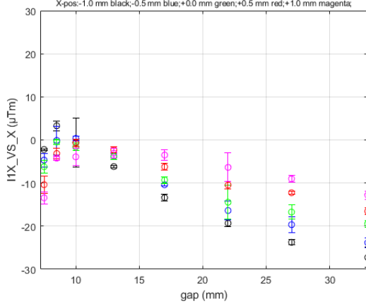
I1X_VS_X for HE_SXU-011 at Long Coil/GoodFieldRegion DATASET0001
