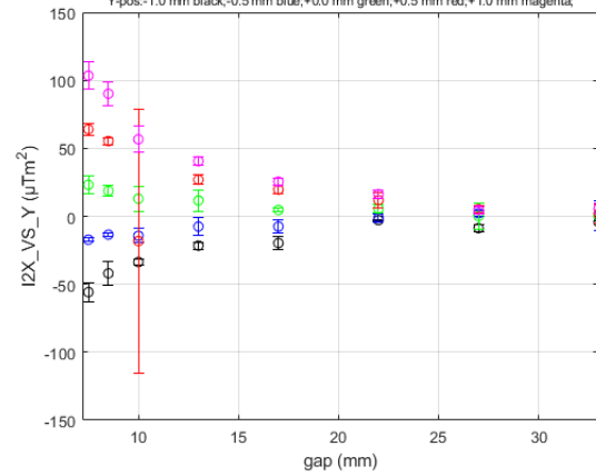
I2X_VS_Y for HE_SXU-011 at Long Coil GoodFieldRegion DATASET0001
