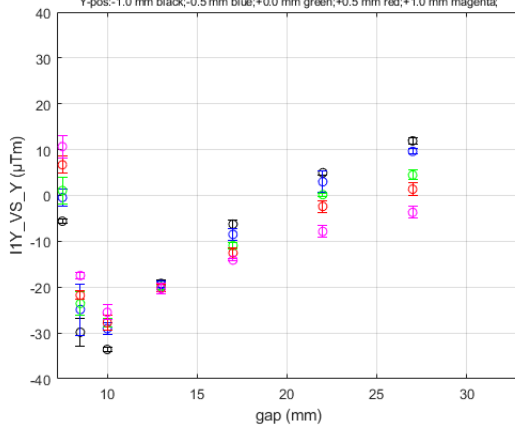
I1Y_VS_Y for HE_SXU-011 at Long Coil GoodFieldRegion DATASET0001
