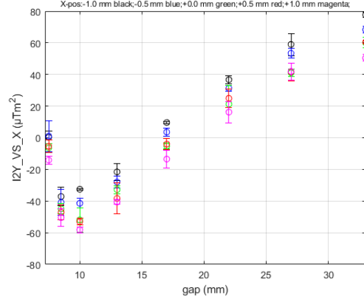
I2Y_VS_X for HE_SXU-011 at Long Coil/GoodFieldRegion DATASET0001
