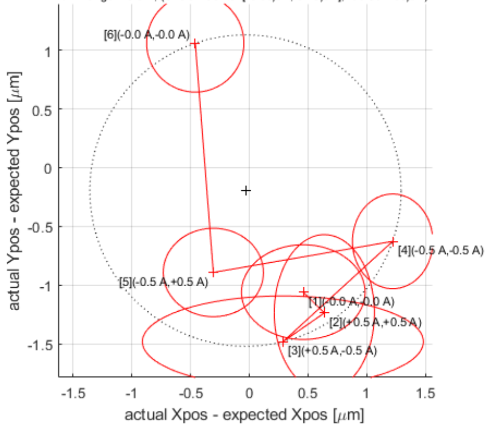
Plot of D Quad Center Motion from XCOR/YCOR: 4269/Final Results/ctrdat.ru4 trim range \pm 0.5 A; (Circle->Center: [-0.03\mu\text{m}, -0.20\mu\text{m}] ; Radius: 1.33\mu\text{m} )
