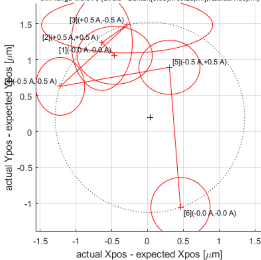
Plot of F Quad Center Motion from XCOR/YCOR: 4269/Final Results/ctrdat.ru4 trim range \pm 0.5 A; (Circle->Center:[0.03 \mu\text{m} , 0.20 \mu\text{m} ]; Radius: 1.33 \mu\text{m} )
