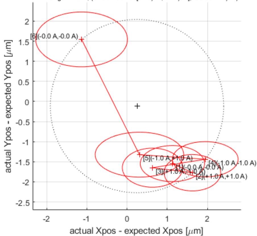
Plot of D Quad Center Motion from XCOR/YCOR: 4269/Final Results/ctrdat.ru3 trim range \pm 1.0 A; (Circle->Center:[0.25 \mu\text{m} , -0.11 \mu\text{m} ]; Radius: 2.16 \mu\text{m} )
