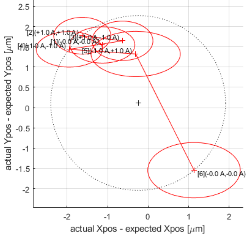
Plot of F Quad Center Motion from XCOR/YCOR: 4269/Final Results/ctrdat.ru3 trim range \pm 1.0 A; (Circle->Center:[ -0.25\mu\text{m} , 0.11\mu\text{m} ];Radius: 2.16\mu\text{m} )
