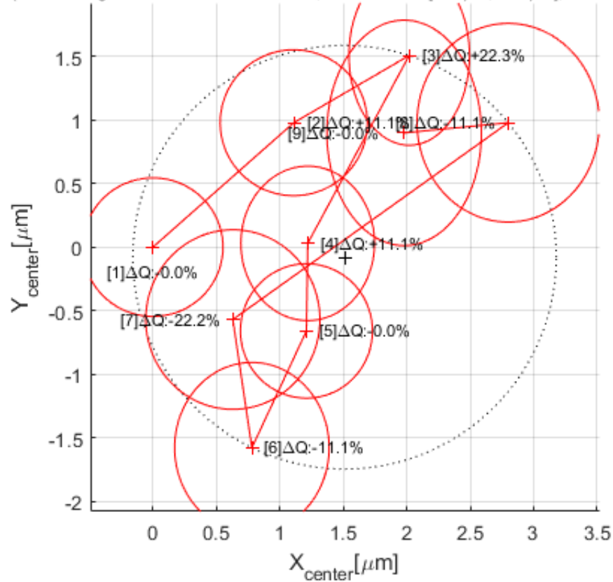
Plot of D Quad Center Position by Quad Strength: 4269/Final Results/ctrdat.ru2 (Quad Strength Modulation around -4.500A; Circle->Center:[1.51 \mu m,-0.08 \mu m];Radius:1.67 \mu m)
