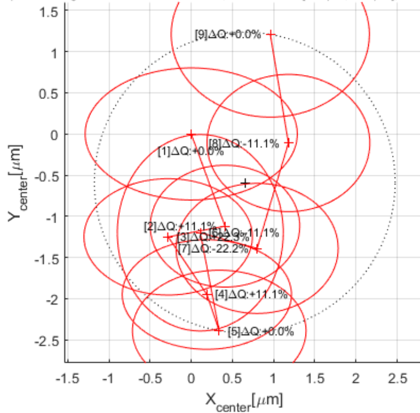
Plot of F Quad Center Position by Quad Strength: 4269/Final Results/ctrdat.ru2 (Quad Strength Modulation around 4.498A; Circle->Center:[0.65 \mu m,-0.59 \mu m];Radius:1.83 \mu m)
