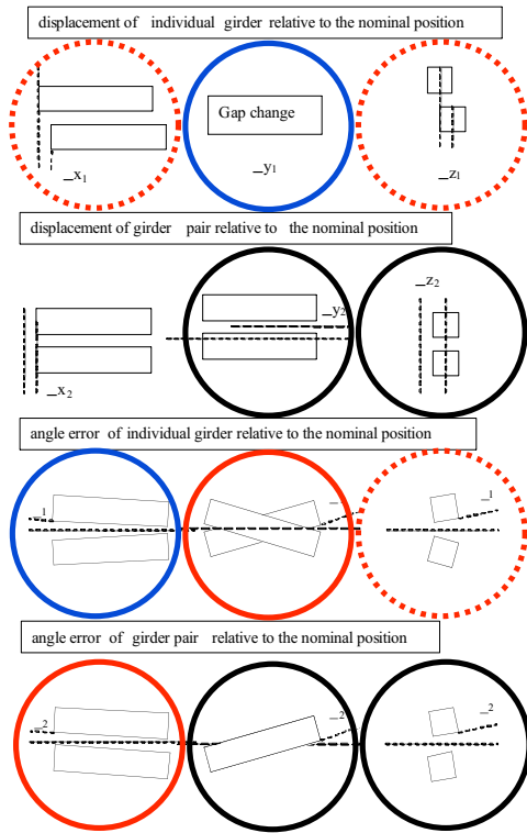
Figure 8: Classification of geometrical tolerances.
