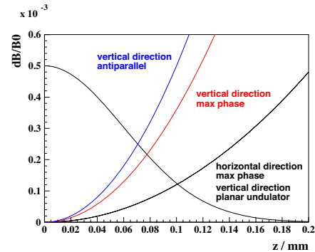
Figure 7: Averaged transverse size of the BESSY FEL electron beam compared to the field roll off for various operation modes.
