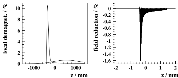
Figure 17: Maximum demagnetization of magnet segments (left) for 1mrad and 0.1mrad angle of incidence and field variation (right) for 1mrad.
