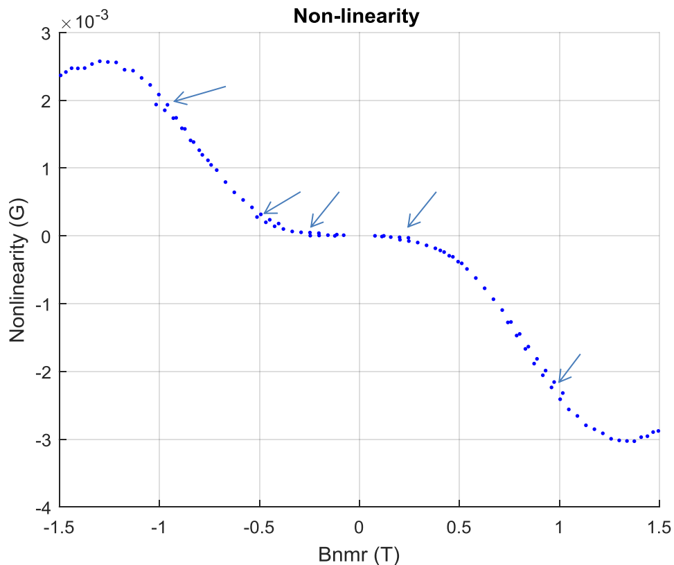
Figure 1. Probe output non-linearity. Zero offset and linear term are subtracted from the measurements. Time between probe changes varies from 1.5hours to 30 minutes.
