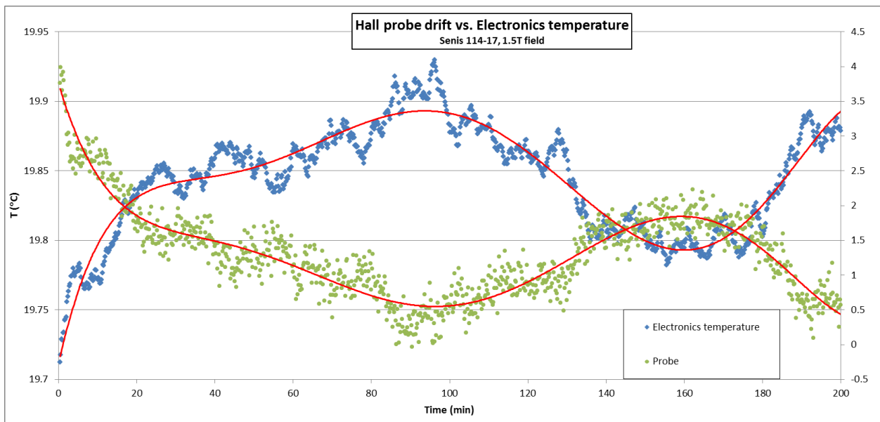
Figure 5. Probe output drift – right axis and the box temperature – left axis.
