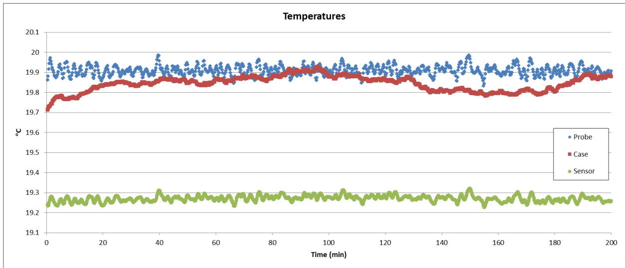
Figure 4. Probe temperature and temperature around the probe are stable but the Box temperature drifts.
