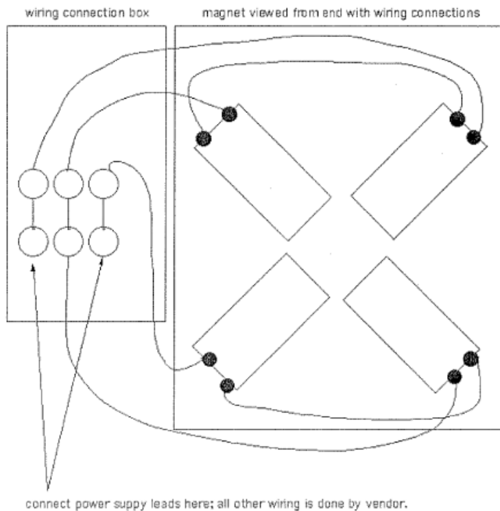
Figure 1. Wiring Scheme
