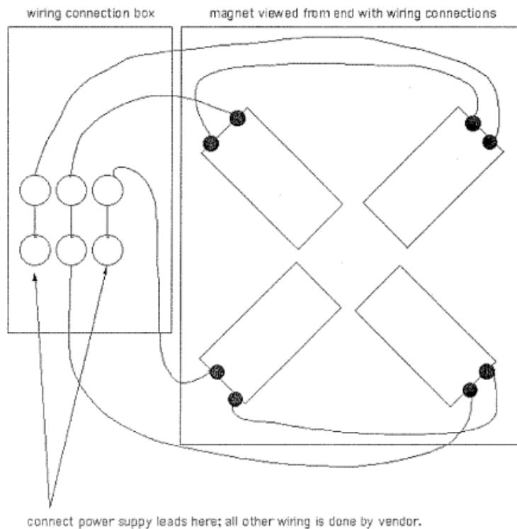
Figure 1. Wiring Scheme
