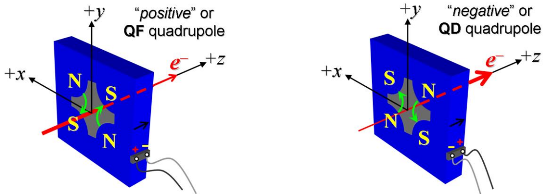
Figure 1. The quadrupoles: QE31B, QE33B, QE35B have “positive” polarity (left), while the quadrupoles: QE32B, QE34B, QE36B have “negative” polarity (right).
