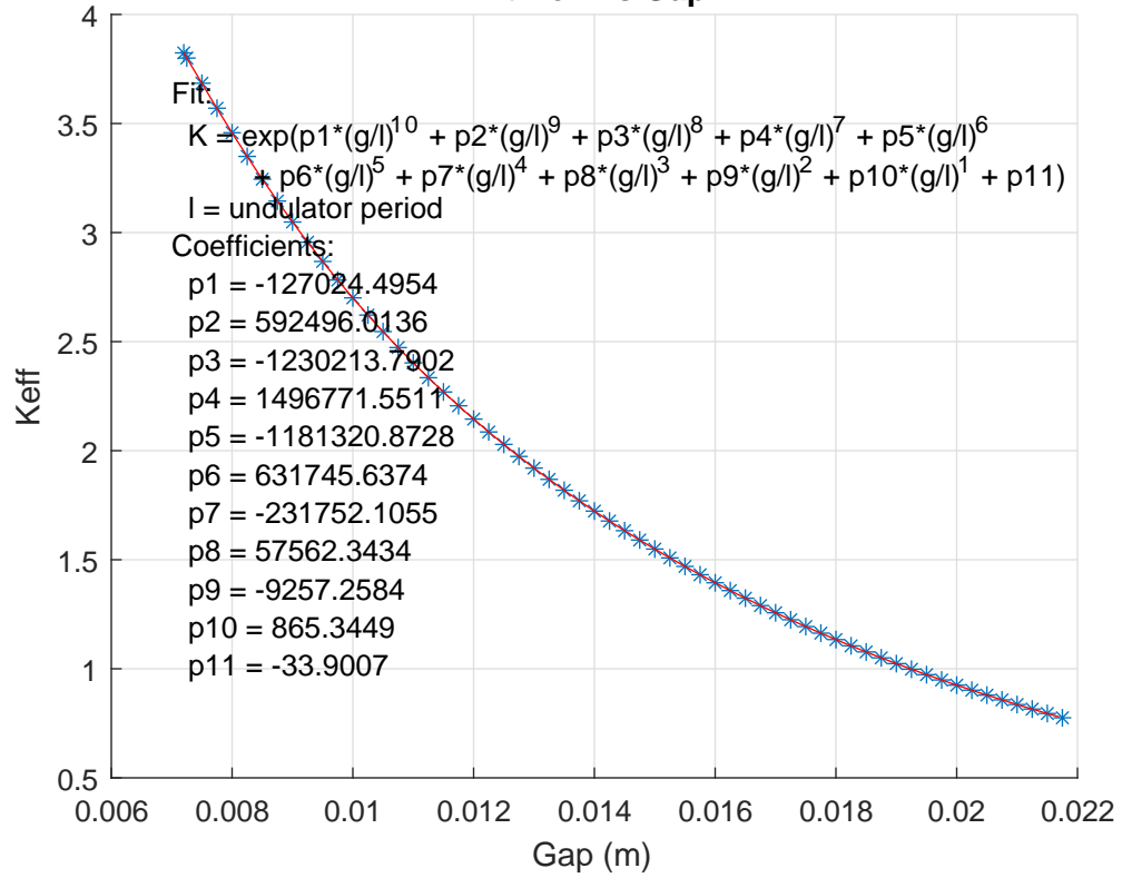
Fit Keff vs Gap
