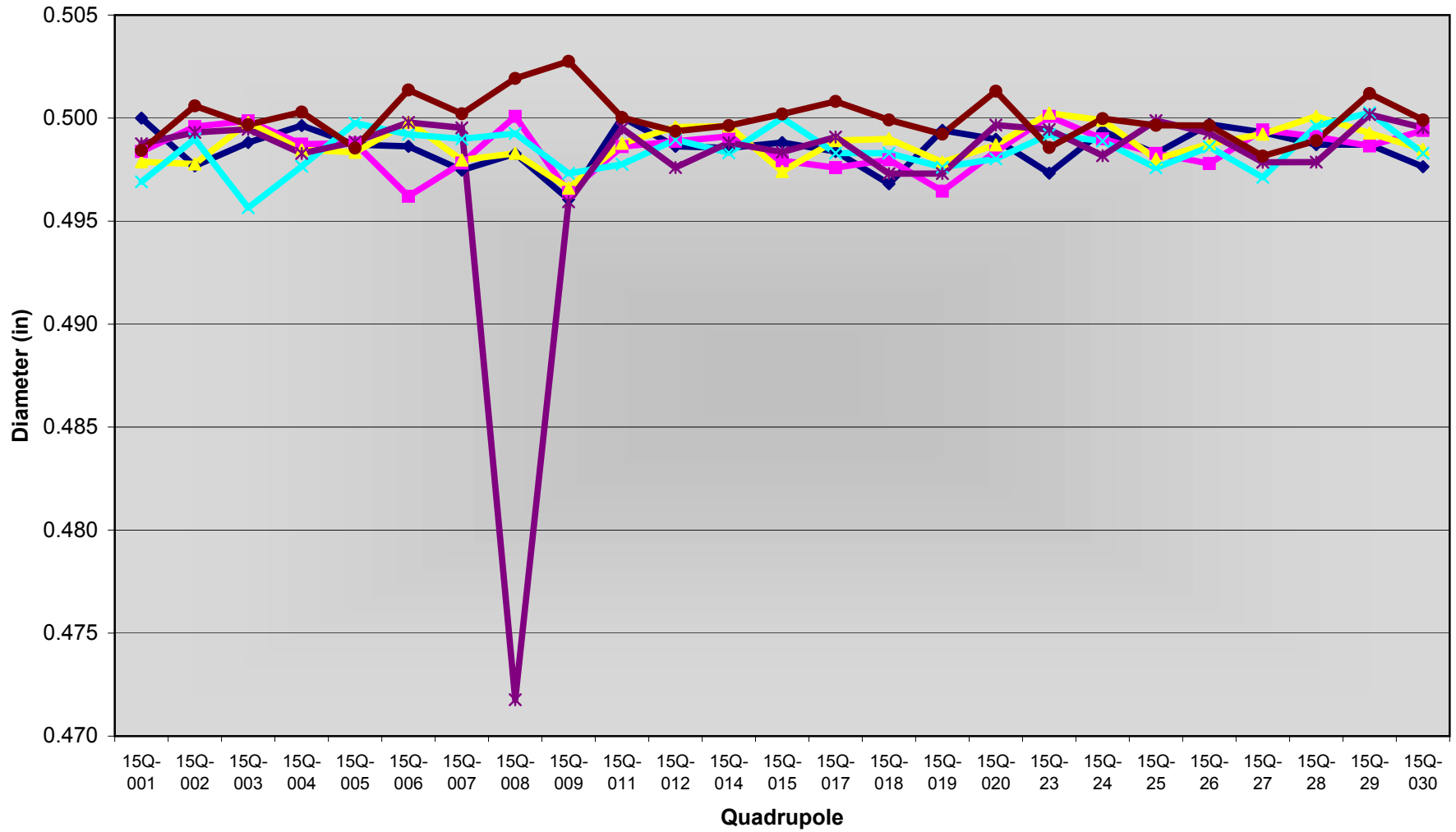
15Q Tooling Ball Diameters
