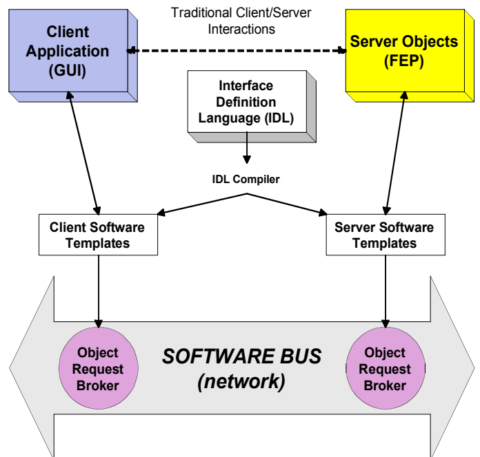
Figure 4: CORBA implements a software bus
