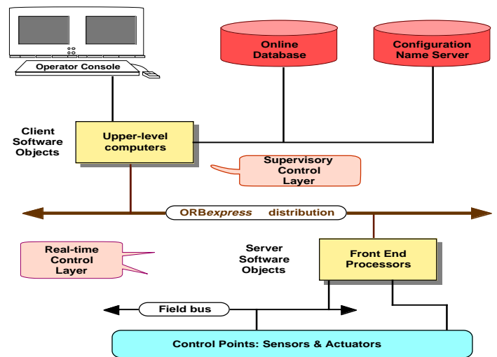
Figure 3: The Supervisor and the Front-end layer communicate using CORBA
